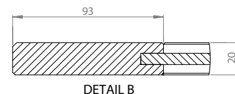
DETAIL B
